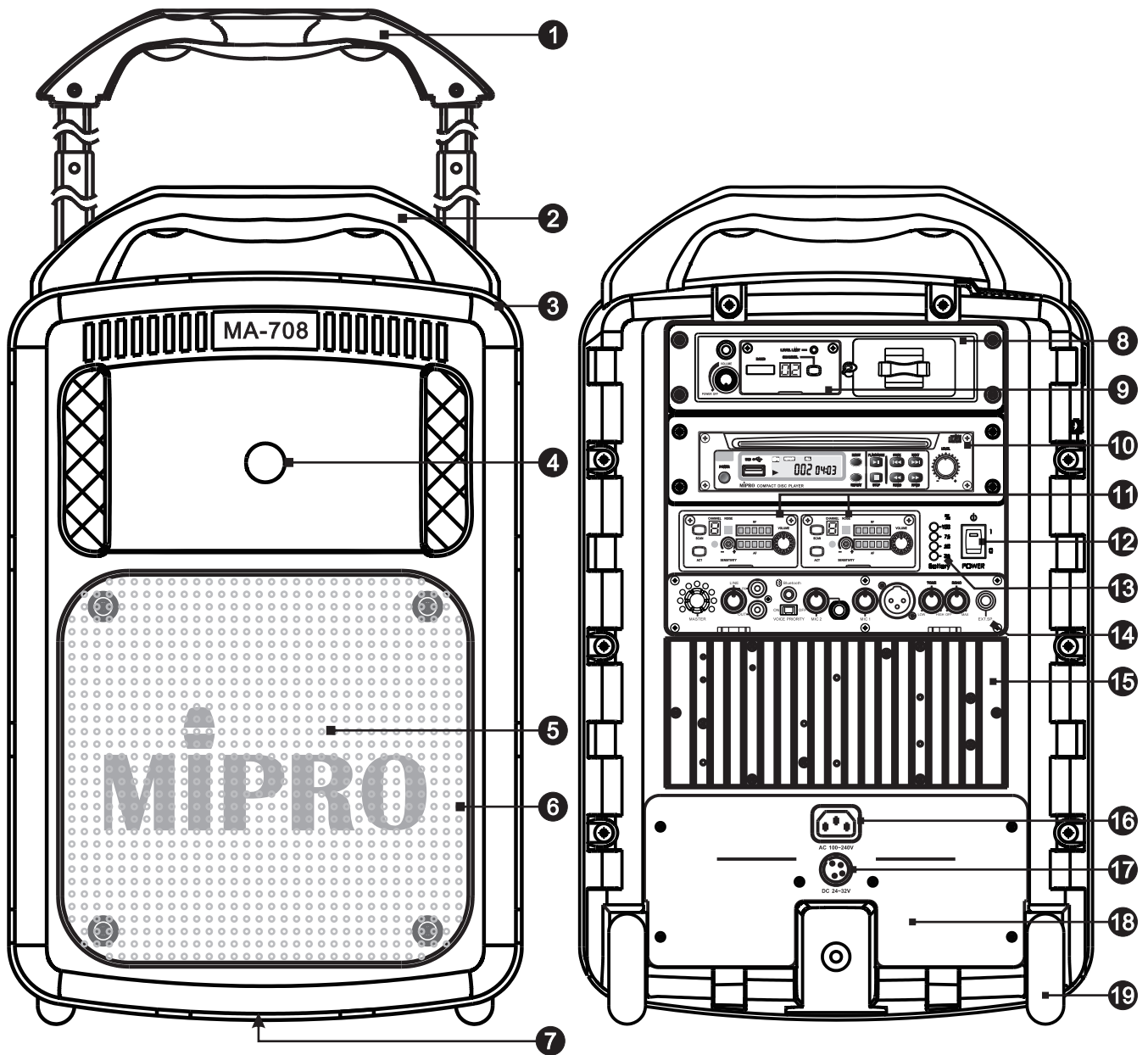
Front Panel
