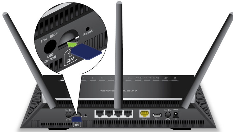
Figure 4. Rear panel
