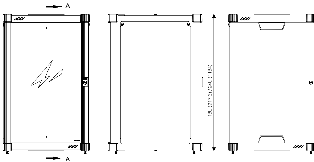
EASYRACK 18U/24U SELF-STANDING (CODE 32252618) (CODE 32252624)
