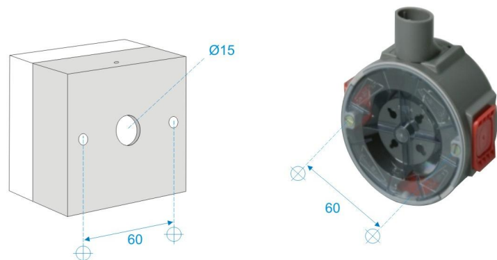
Fixture will cover and screw-mounting-holes fits on wallbox
