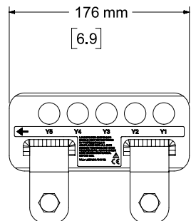
Left View
